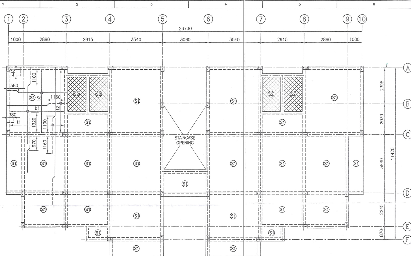
FIRST FLOOR SLAB LAYOUT (T.O.C (+)3.55M) (SCALE 1:100)
